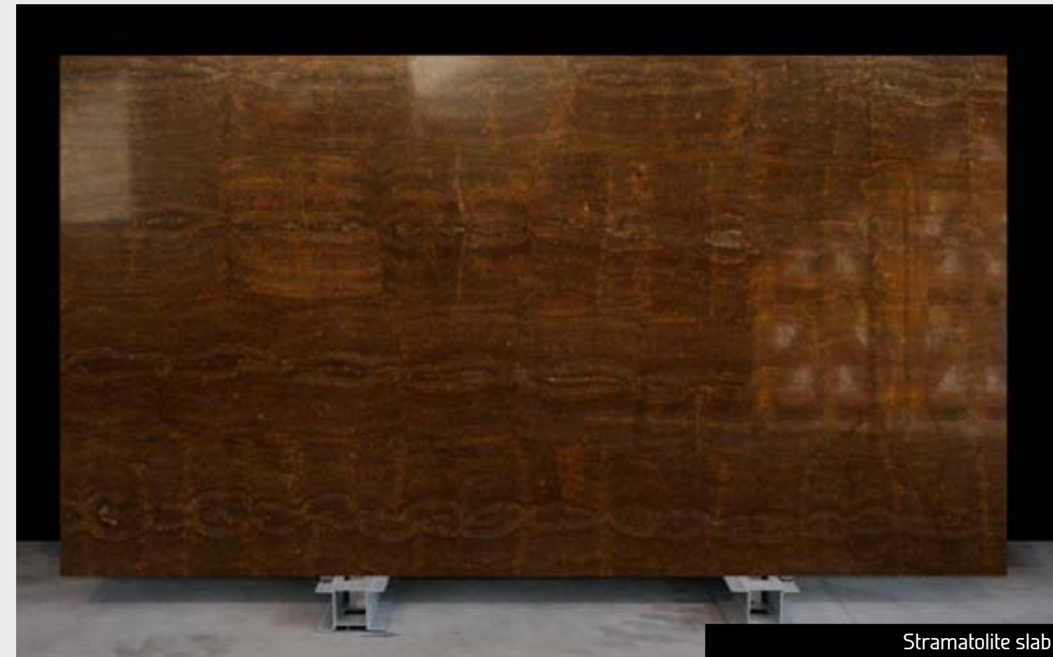
Stramatolite random slab
